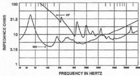
FIGURE 2 — MTH-2.5/94B Impedance vs. Frequency
