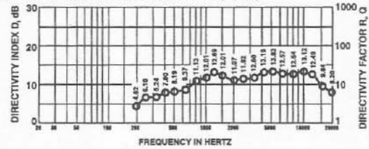
FIGURE 6 — MTH-2.5/94B Harmonic Distortion
