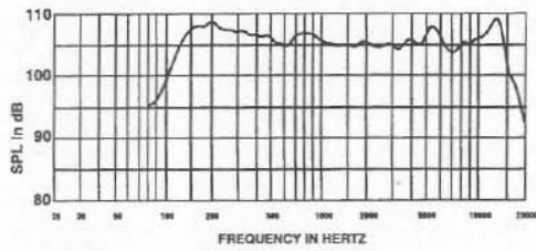
FIGURE 1 — MTH-2.5/94B Axial Frequency Response
