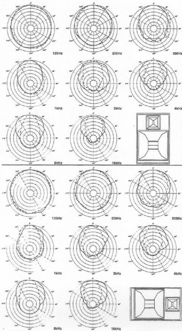
FIGURE 3 — MTH-2.5/94B Polar Response
