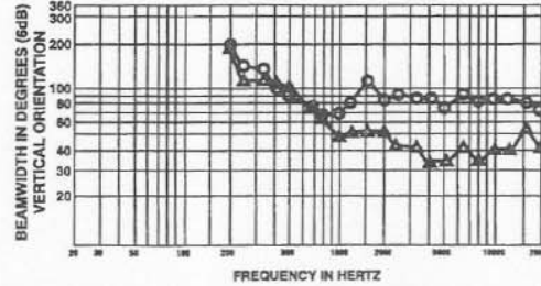
FIGURE 4 — MTH-2.5/94B Beamwidth vs. Frequency
