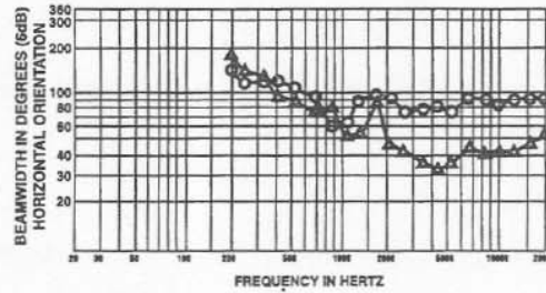
FIGURE 5 — MTH-2.5/94B Directivity vs. Frequency
