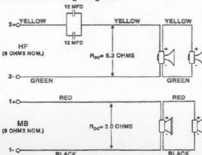
FIGURE 7 — MTH-2.5/94B Wiring Diagram
